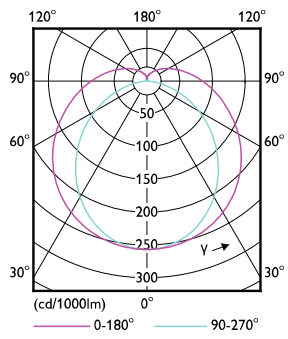
TLED_4ft_220-240V15.5-36W_G13-LDD
