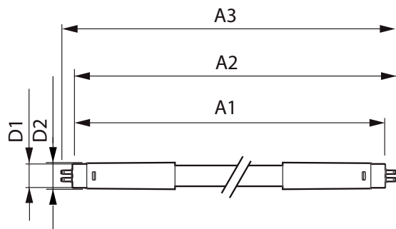
TLED 1500mm 230V17W-35W 2600lm 160D 650
