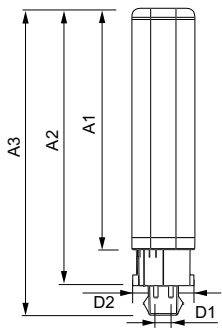
PLED PLC 120V 8.5-26W 950lm 3500K GX24q
