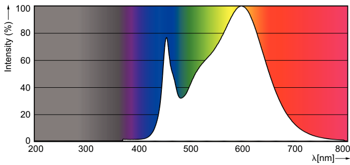
LEDtube 1200mm 15W G13 T8 835 2000lm
