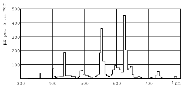
LDPB_TL-D8LL_830-Spectral power distribution B/W
