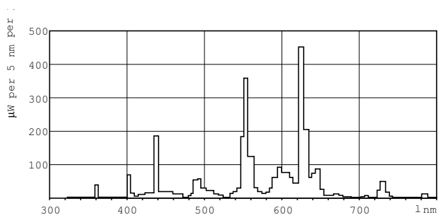
LDPB_TL5-HE8_830-Spectral power distribution B/W
