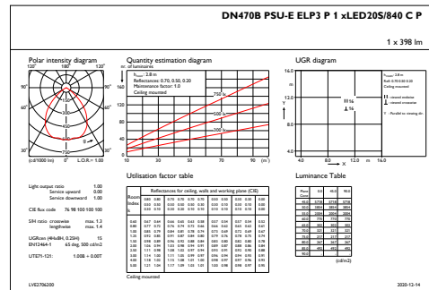
IFGU1_DN470BPSU-EELP3P1xLED20S840CP
