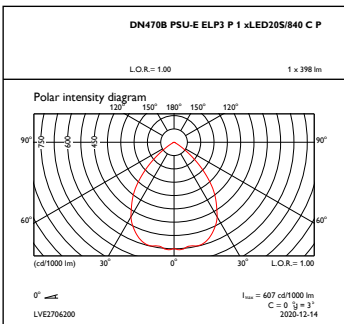
OFPC1_DN470BPSU-EELP3P1xLED20S840CP
