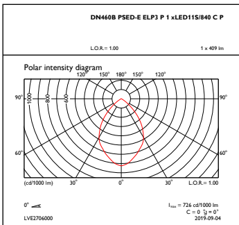
OFPC1_DN460BPSED-EELP3P1xLED11S840CP
