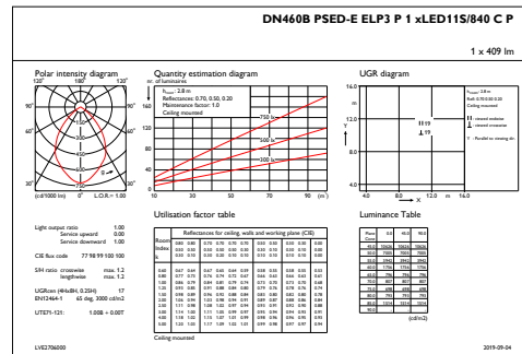
IFGU1_DN460BPSED-EELP3P1xLED11S840CP
