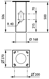
OptiSpace bollard acc. ZCB500
