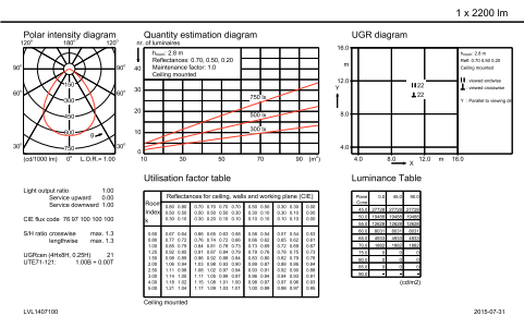
DN570B PSE-E 1xLED20S/830 F
