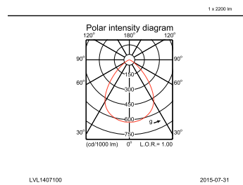
DN570B PSE-E 1xLED20S/830 F
