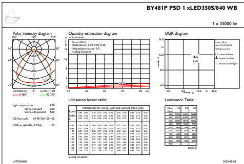
IFGU1_BY481PPSD1xLED350S840WB
