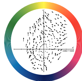
LDCR_CDM-T_150W_830-Colour rendering diagram
