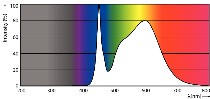
Spectral Power Distribution Colour - MAS LEDtube 1050mm 14W840 T8 TW
