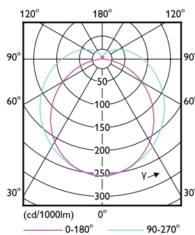
Light Distribution Diagram - MAS LEDtube 1050mm 14W840 T8 TW
