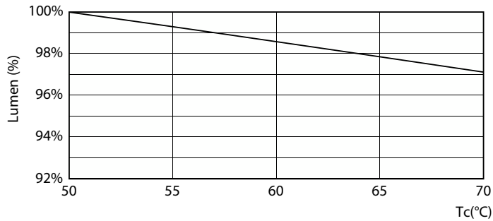
Lumen Maintenance Diagram - MAS LEDtube 1200mm HO 14W865 T8 MY
