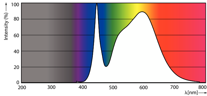
Spectral Power Distribution Colour - CorePro LEDtube 1500mm 20W 840 T8 CL
