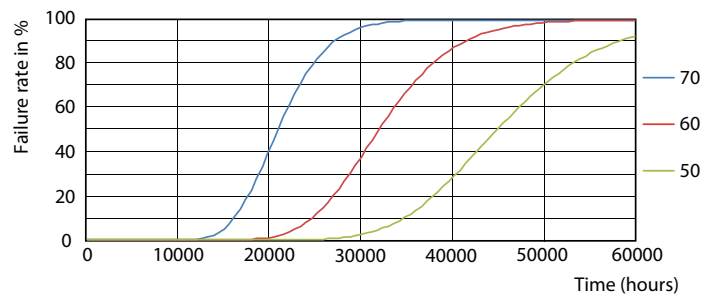
Life Expectancy Diagram - CorePro LEDtube HO 1200mm 18W865 VWV T8
