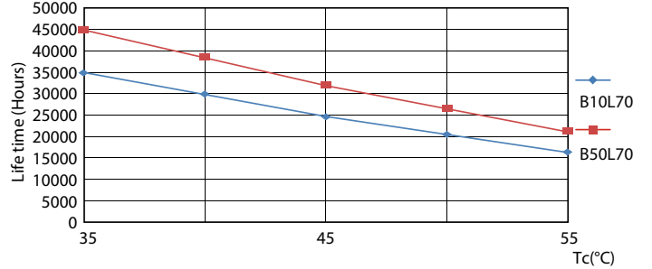
Life Expectancy Diagram - CorePro LEDtube 600mm 9W 840 T8 AP I
