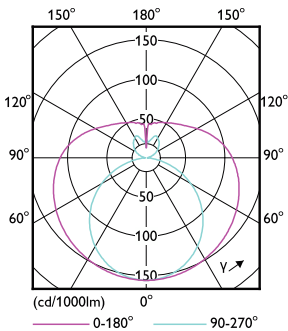
Light Distribution Diagram - CorePro LEDtube 600mm 9W 840 T8 AP I
