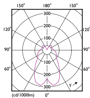
Light Distribution Diagram - MAS LEDlustre DT 2.8-25W E14 P48 CL
