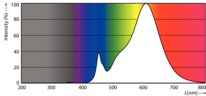
Spectral Power Distribution Colour - MAS LEDlustre DT 2.8-25W E14 P48 CL
