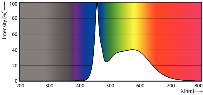
LEDtube MAS GM 20,5W G13 3300lm 865-POC
