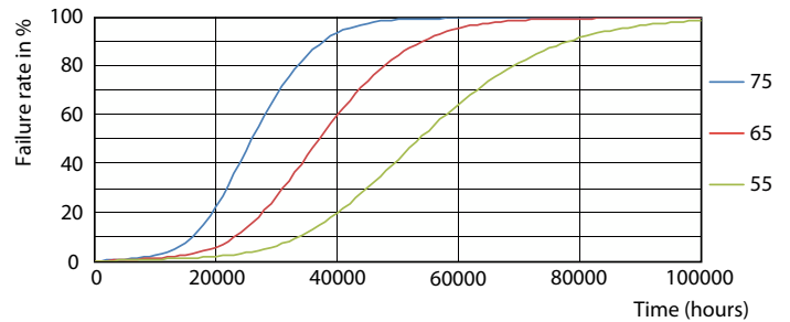
Life Expectancy Diagram - Master LEDTube 1200mm 15.5W 840 T8 W JP
