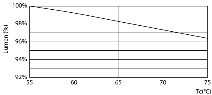
Lumen Maintenance Diagram - Master LEDTube 1200mm 15.5W 840 T8 W JP
