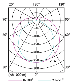
Light Distribution Diagram - Master LEDTube 1200mm 15.5W 840 T8 W JP
