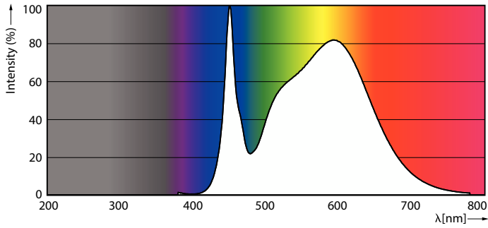
Spectral Power Distribution Colour - Master LEDTube 1200mm 15.5W 840 T8 W JP
