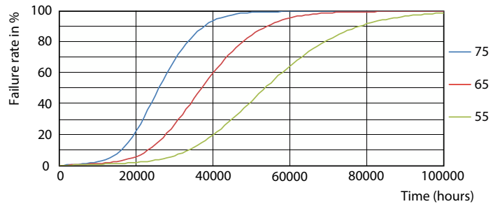
Life Expectancy Diagram - Master LEDTube 1200mm 12.5W 865 T8 W JP
