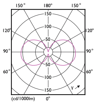
Light Distribution Diagram - LEDClassic 6W ST64 E27 830 CLND1PF/10
