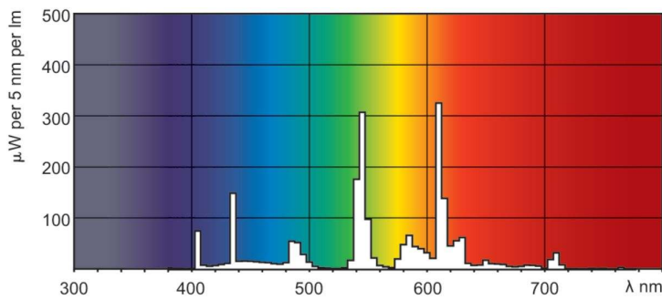
Spectral Power Distribution Colour - PL-T 42W/835/XEW/A/4P/33W 1CT/5X10 ALTO
