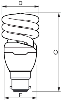
TORNADO 15W WW B22 220-240V 1PF/6
