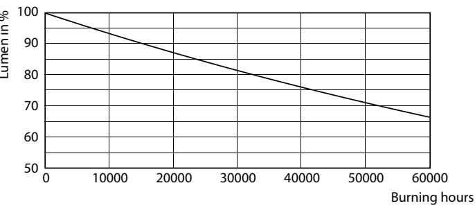
Lumen Maintenance Diagram - 11T8/COR/48-840/MF16/G/BAA 25/1
