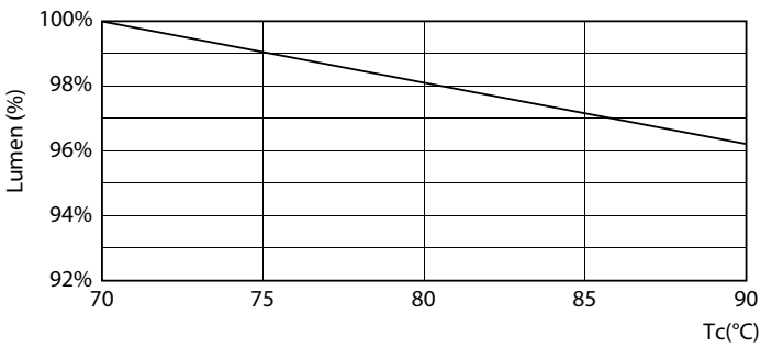
Lumen Maintenance Diagram - 11T8/COR/48-840/MF16/G/BAA 25/1
