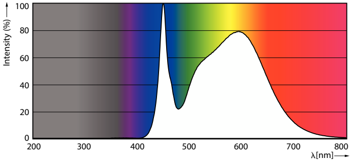
Spectral Power Distribution Colour - 11T8/COR/48-840/MF16/G/BAA 25/1
