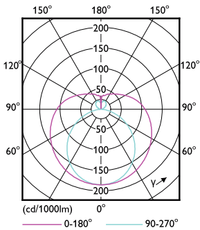
Light Distribution Diagram - 11T8/COR/48-840/MF16/G/BAA 25/1
