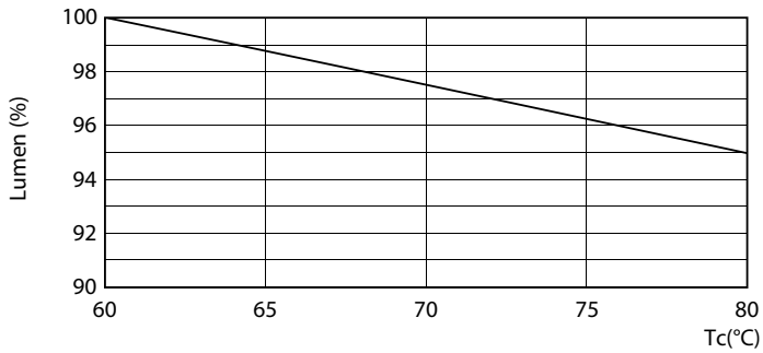
Lumen Maintenance Diagram - Ledtube DE 1200mm 18W 765 T8 TH 3SL
