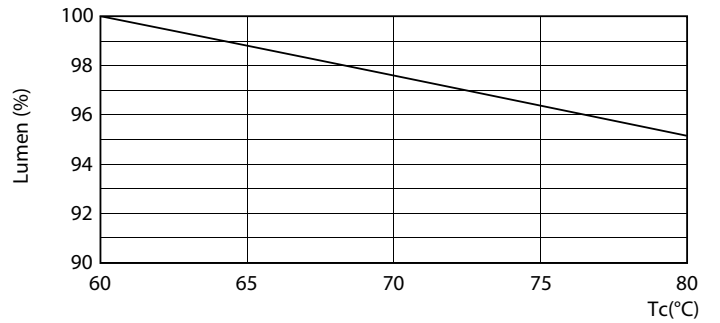
Lumen Maintenance Diagram - Ledtube DE 600mm 9W 900lm 765 T8 G13 C
