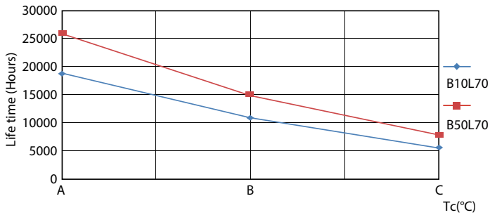
Life Expectancy Diagram - Ledtube DE 600mm 9W 900lm 765 T8 G13 C
