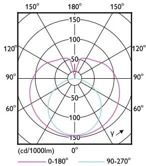
Light Distribution Diagram - Ledtube DE 600mm 9W 900lm 765 T8 G13 C
