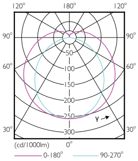
Light Distribution Diagram - MAS LEDtube 1200mm UO 16W 865 T8 FF RCA
