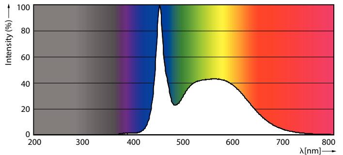
Spectral Power Distribution Colour - MAS LEDtube 1200mm UO 16W 865 T8 FF RCA
