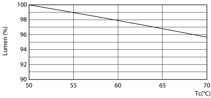
Lumen Maintenance Diagram - MAS LEDtube 1200mm UO 16W 865 T8 FF RCA
