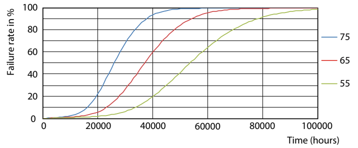
Life Expectancy Diagram - MAS LEDtube 1200mm UO 16W 865 T8 FF RCA
