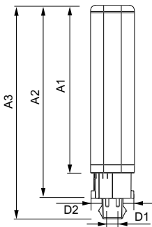
12PL-C/T/COR/32H-835/IF14/P/4P/DIM 10/1
