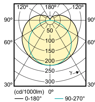
MASTER LEDtube HF 1200mm 16.5W G13 3300K 960lm T8
