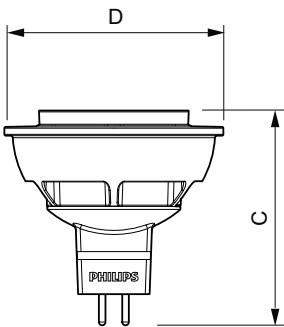
MASTER LED 5.5-50W 2700K MR16 24D CN
