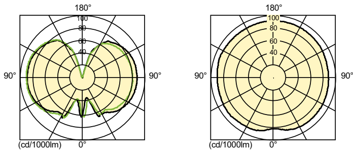
Light Distribution Diagram - CDM T12 ELITE 315W/942/U/O GAV
