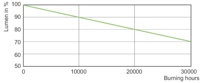
Lumen Maintenance Diagram - CDM T12 ELITE 315W/942/U/O GAV
