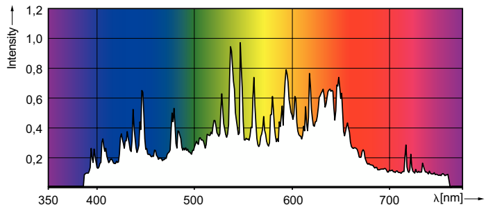
Spectral Power Distribution Colour - CDM T12 ELITE 315W/942/U/O GAV
