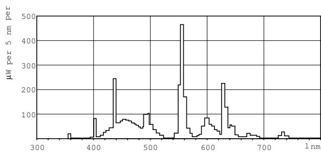
LDPB_TL5ECO_865-Spectral power distribution B/W
