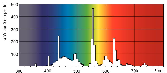
LDPO_TL5ECO_865-Spectral power distribution Colour
