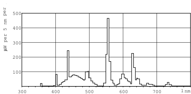
LDPB_TL-D8LL_865-Spectral power distribution B/W
