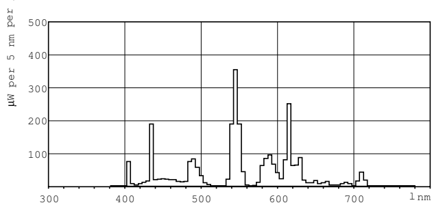
LDPB_TL-D8_835-Spectral power distribution B/W
