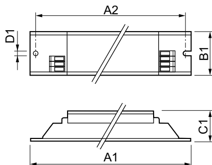
EB-P 254/255/258 TL-D/PL-L/TL5HO
