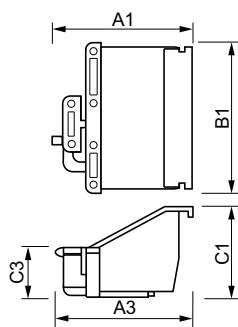
HID-STRAIN RELIEF
