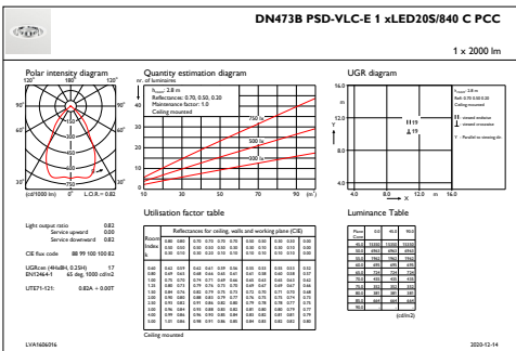
IFGU1_DN473BPSD-VLC-E1xLED20S840CPC
