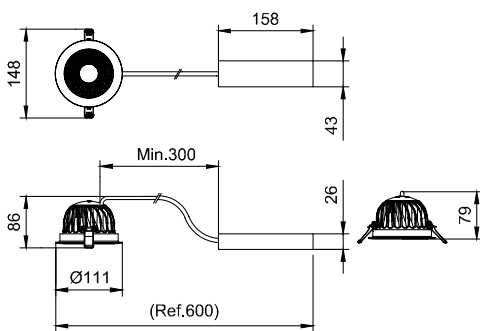
DN588B LED6/840 PSU C D100 WH WB GC
