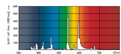
MASTER HPI-T Plus 400W
